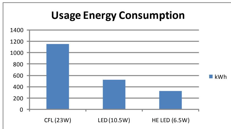
Figure 4: Comparison of CFL to Cree LR6 LED and High-Efficiency LR6 LED lifetime energy usage in a recessed downlight application (50,000 hours at equivalent lumens output).
