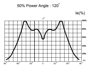
FIG.6 FAR FIELD PATTERN
