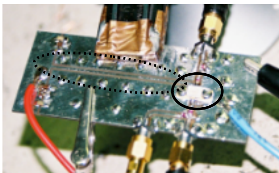
Fig. 5. The PCB with the transmission line indicated by the dashed ellipse and the device by the solid one.
