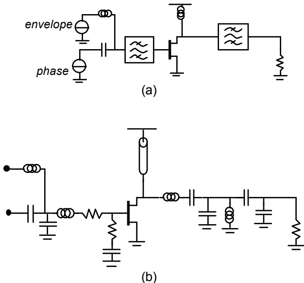
Fig. 3. Power amplifier schematic, (a). Block diagram, (b). Implementation.
