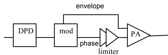
Fig. 1. Transmitter architecture.
