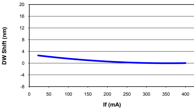
Wavelength Shift vs. Forward Current
