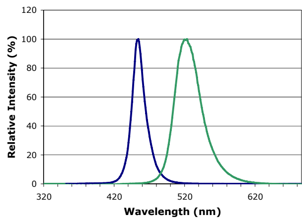
Relative Intensity vs Peak Wavelength
